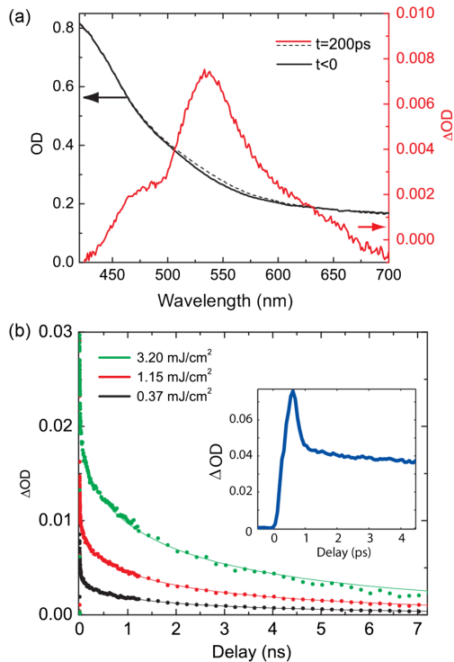
FIG. 2 (color online). (a) Optical absorption spectra in units of the optical density (OD) before (solid line) and after (dashed line) optical excitation of BFO film at absorbed fluence of 3.2 \text{ mJ/cm}^2 . The red curve shows the change in optical density ( \Delta\text{OD} ) at 200 ps. (b) Transient absorption at 540 nm as a function of delay at various absorbed fluences from 0.37 to 3.2 \text{ mJ/cm}^2 . The solid lines represent the fits using a biexponential decay. The inset shows the initial ps dynamics at the absorbed fluence of 3.2 \text{ mJ/cm}^2 .
