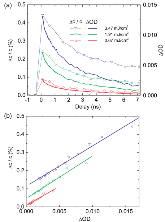
FIG. 3 (color online). (a) The dynamics of the induced strain (triangles and diamonds) and optical absorption (solid lines) interpolated from Fig. 2(b) at various absorbed fluences from 0.67 to 3.47 \text{ mJ/cm}^2 . (b) Strain as a function of the induced absorption at various fluences. The solid lines are linear fits.
