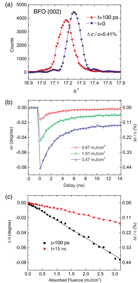
FIG. 1 (color online). (a) \theta - 2\theta scans of the BFO 002 Bragg reflection before and 100 ps after excitation by a 50 fs laser pulse with a central wavelength of 400 nm and the absorbed fluence of 3.2 \text{ mJ/cm}^2 . (b) The angular shift \Delta\theta of Bragg peaks and induced strain as a function of delay at various absorbed fluences from 0.67 to 3.47 \text{ mJ/cm}^2 . The solid lines represent fits of a biexponential decay. (c) The angular shift and induced strain as a function of the absorbed fluence at 100 ps and 15 ns after the excitation. The solid lines represent linear fits.
